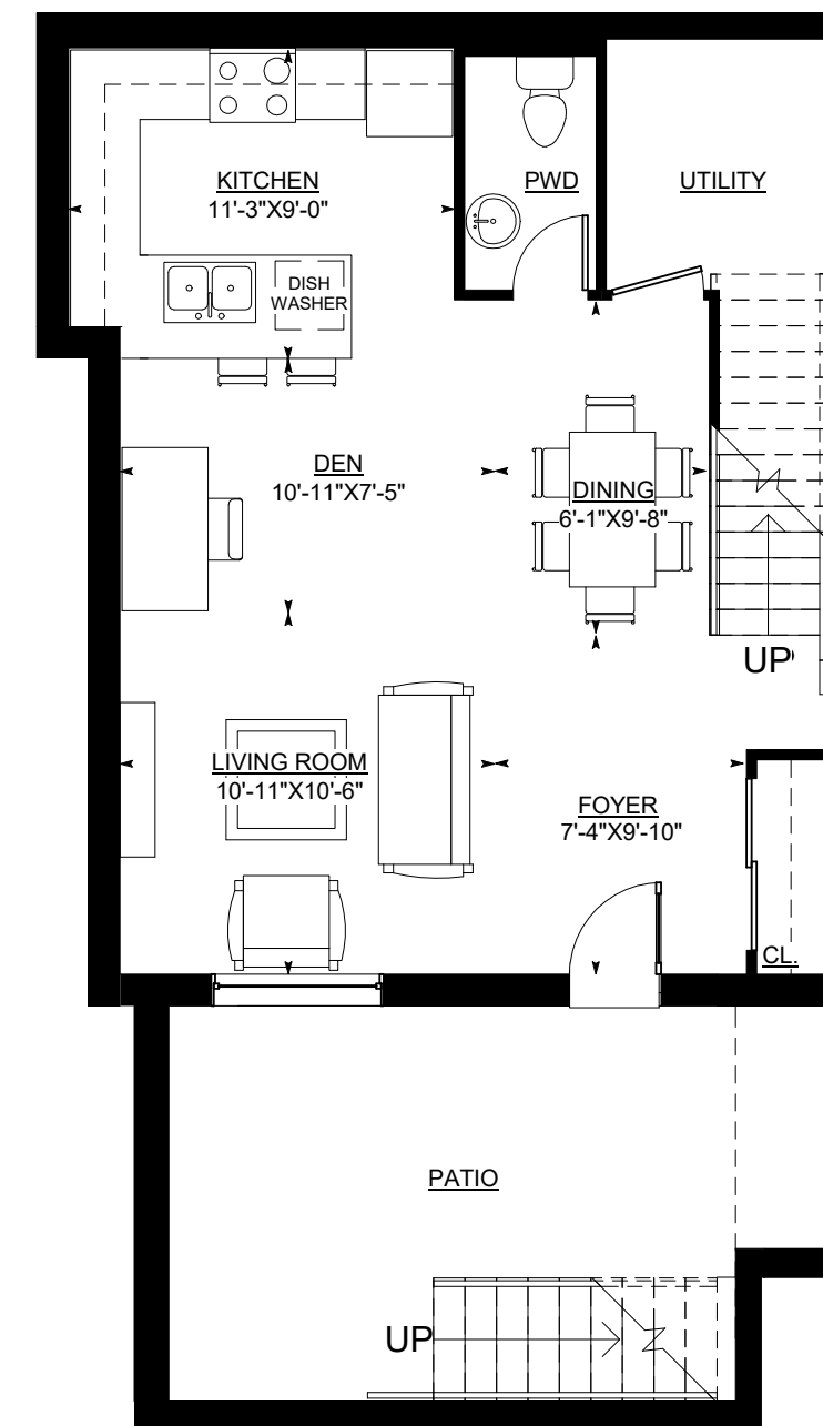
MAIN FLOOR
