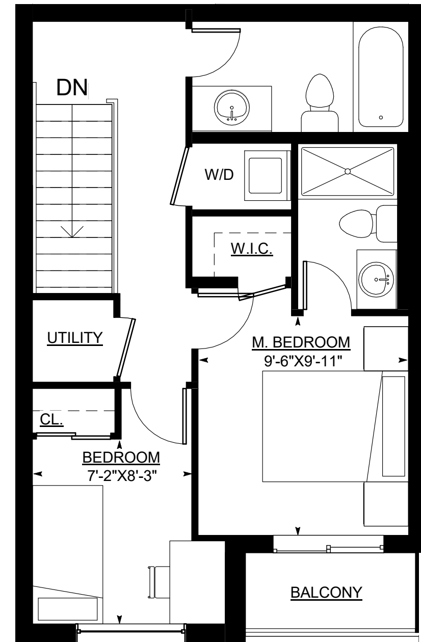
UPPER FLOOR
